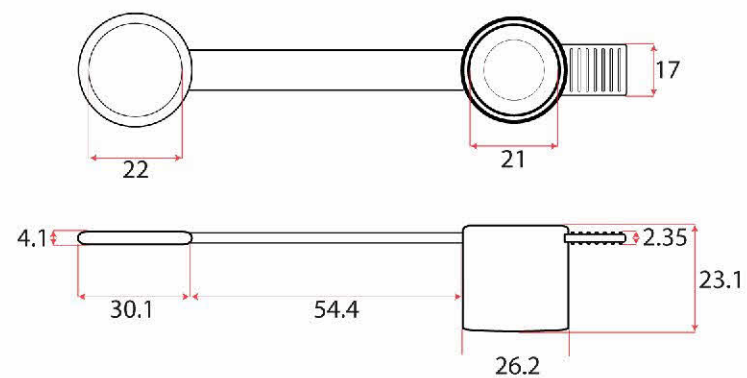
COVERING CAP
